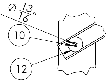
DETAIL C SCALE 1 : 15
