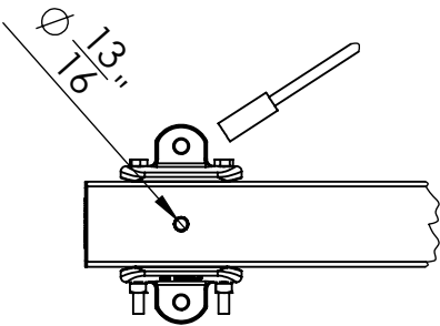
DETAIL D SCALE 1 : 15
