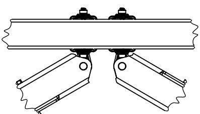
DETAIL E SCALE 1 : 15
